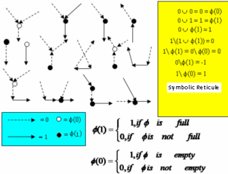
FIGURE 9.5 The Quantum logic algebra and their symbolic reticule [J2]
