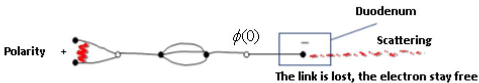
FIGURE 9.6 The corresponding anomalous string graph [28, 29]
